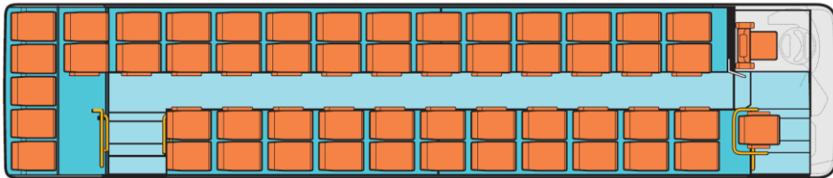
Layout 12 m: 53 places + hostess
