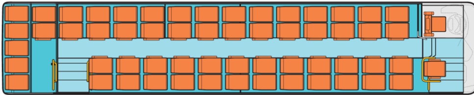
Layout 13 m: 57 places + hostess
